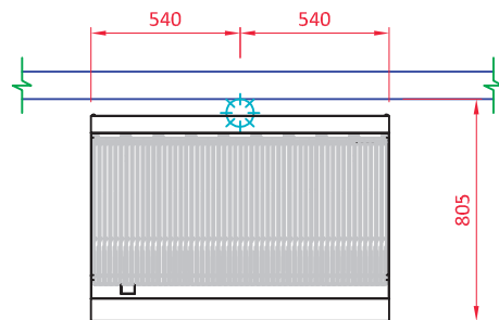
VISTA FRONTAL
