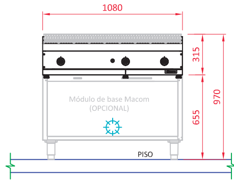
VISTA FRONTAL
