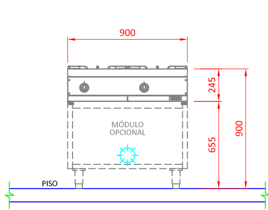
VISTA FRONTAL
